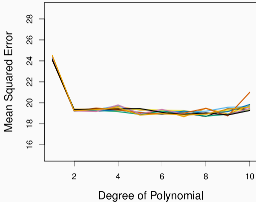
10-fold CV
